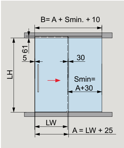
Single panel with sidelight, running / closing on 90° wall
