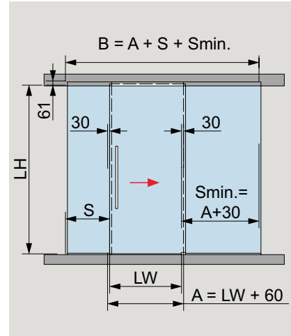
Single panel in ceiling, with two sidelights
